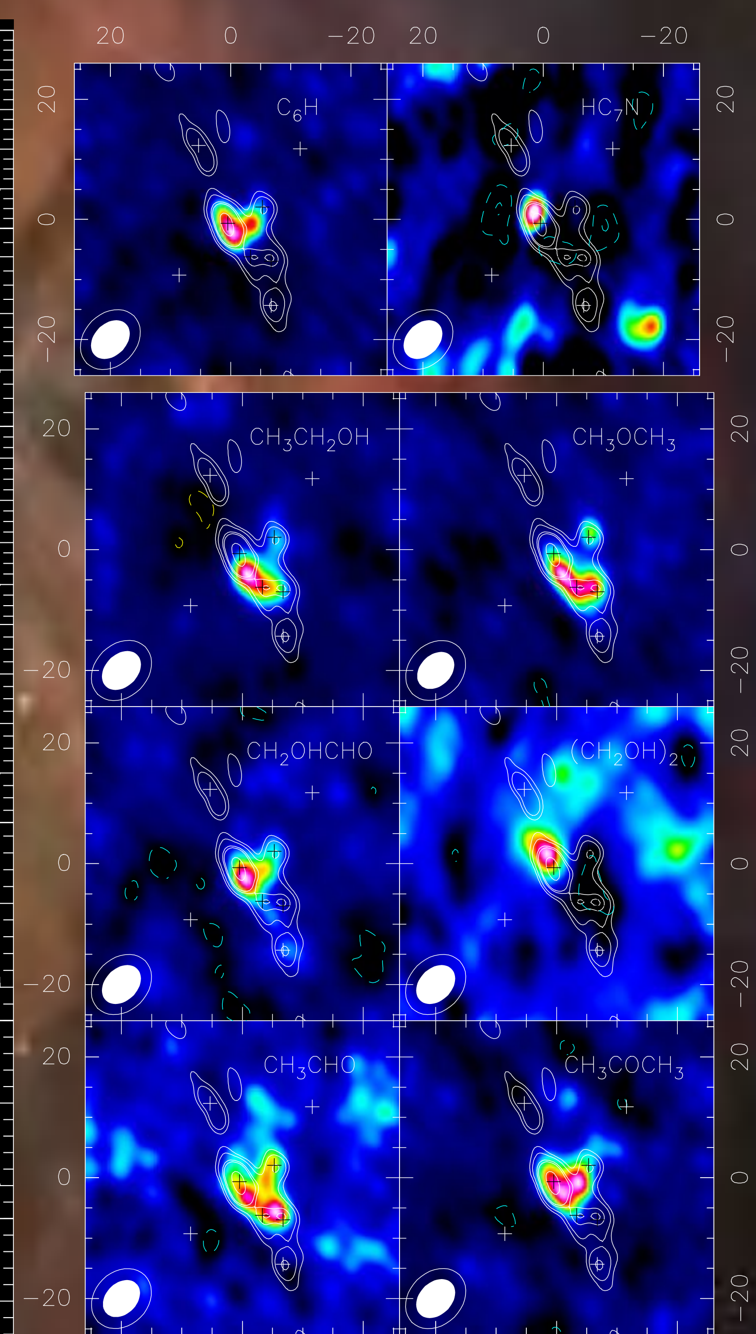
Fig.5. Spatial distribution for the identified ( CH3COCH3 , CH3CH2OH , CH3OCH3 ) and tentative [ HC7N , C6H , CH2OHCHO , CH3CHO , (CH2OH)2 ] COMs.
